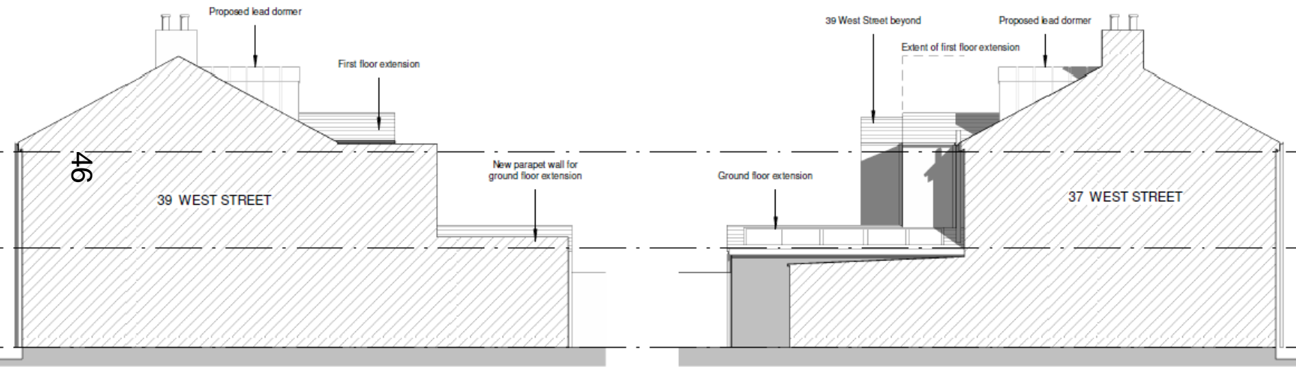
South Elevation
