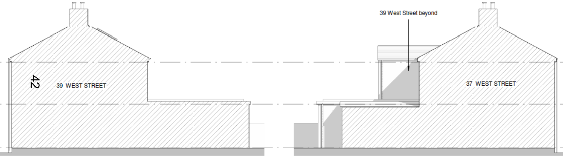
North (side) Elevation
